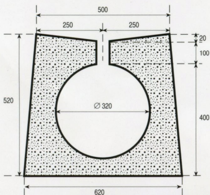
CAZ "IN SITU"
