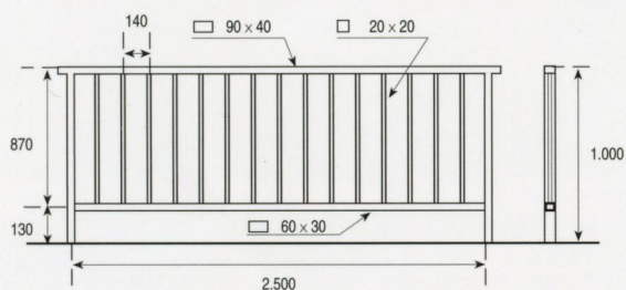
BARANDA PEATONAL STANDARD
